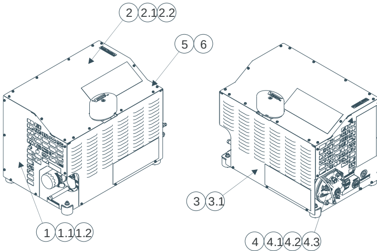
Figure 6 – Panel Assembly
