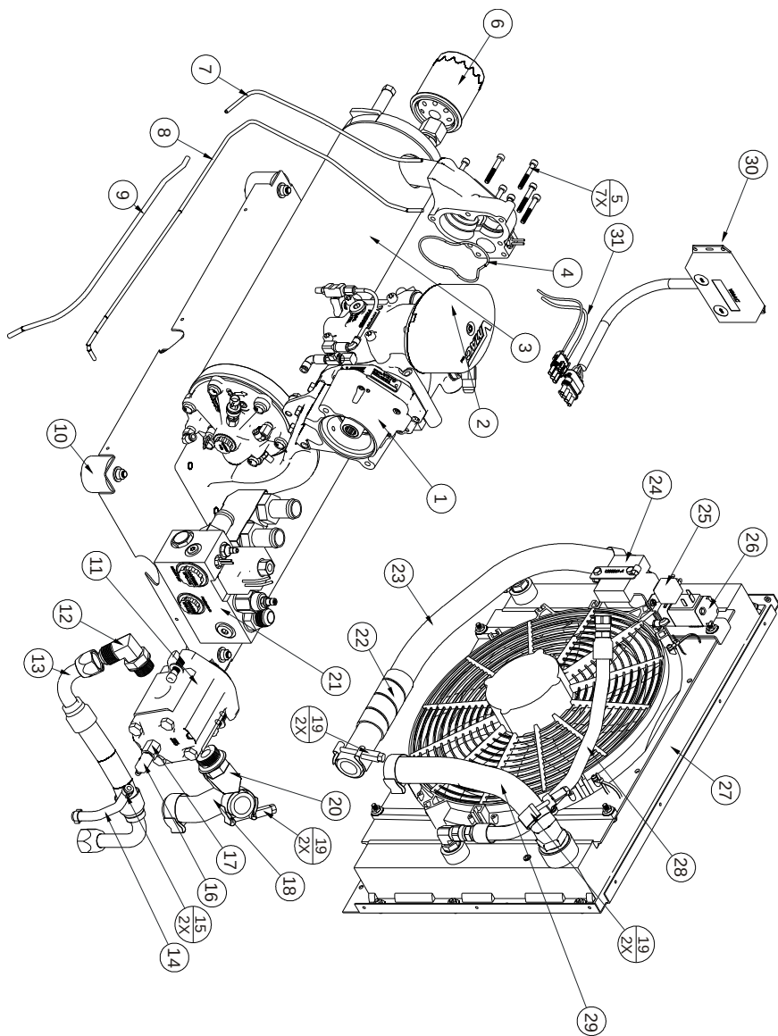
Figure 1 – Main Assembly
