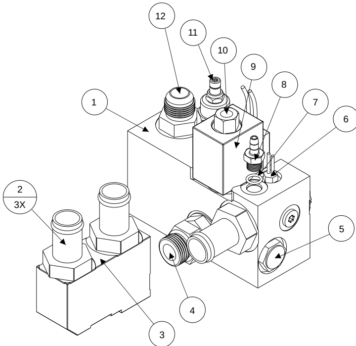
Figure 4 – Manifold Assembly
