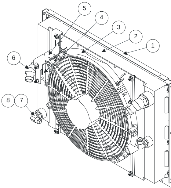
Figure 3 – Cooler Assembly
